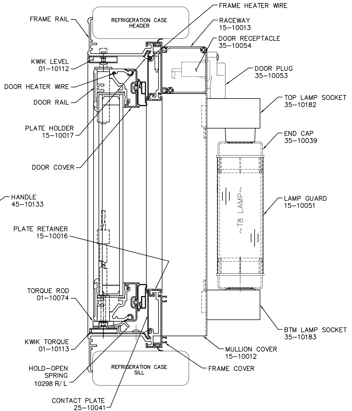
COMMERCIAL DISPLAY SYSTEMS PARTS IDENTIFICATION
