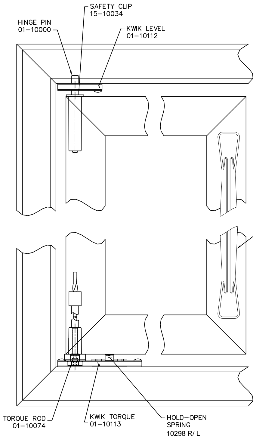
COMMERCIAL DISPLAY SYSTEMS PARTS IDENTIFICATION
