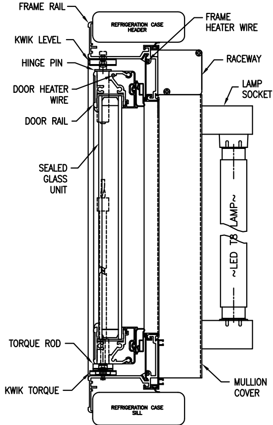
LEGACY SERIES SIDE CROSS SECTION
